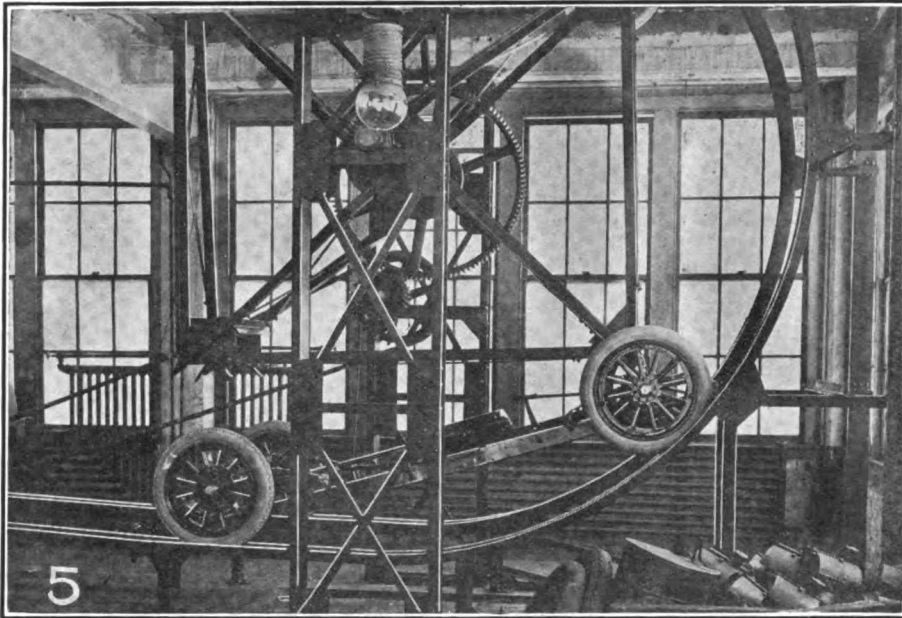
5 Chassis lifted to second floor and to upright position by Ferris wheel device
